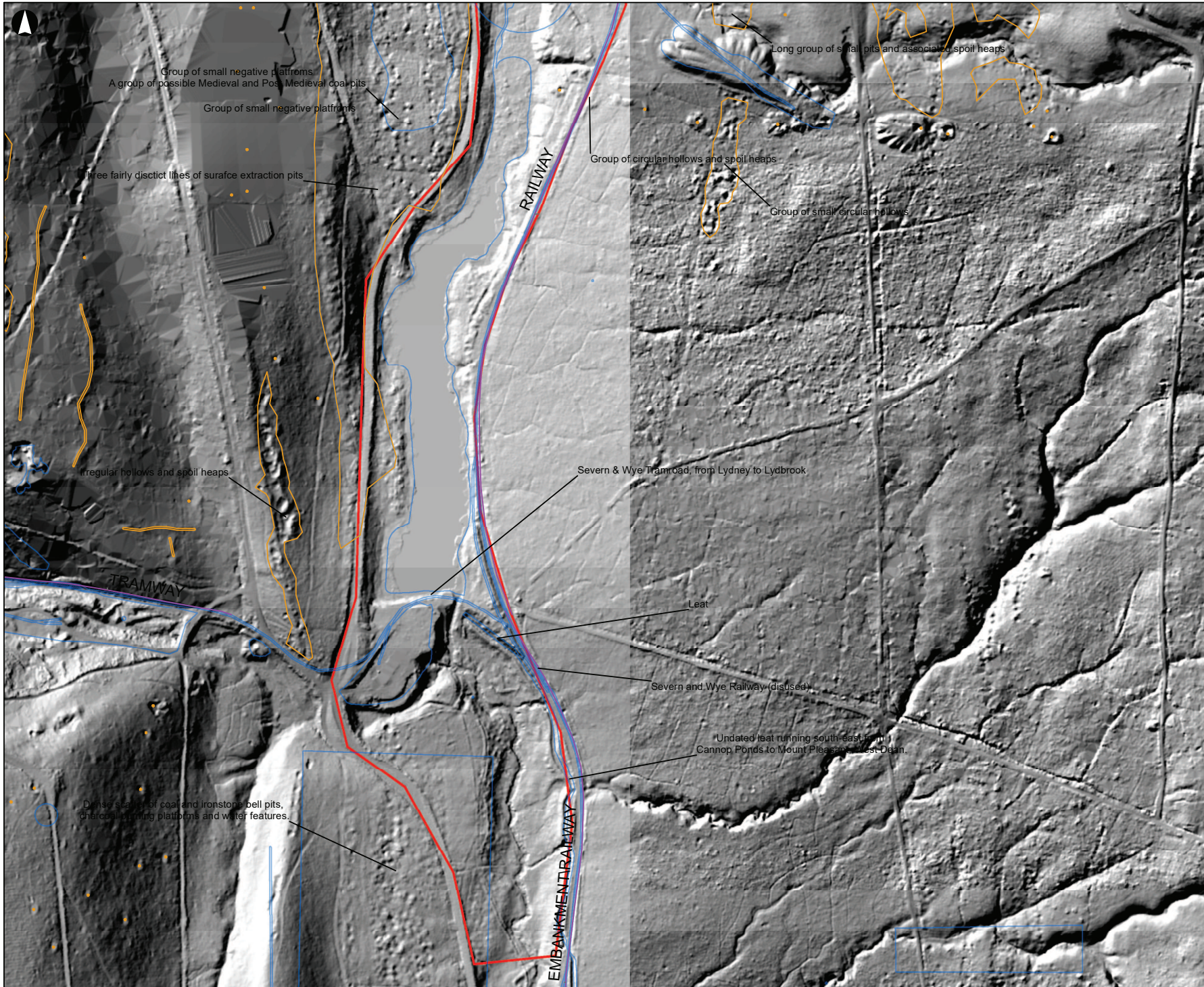
Figure 10: Lidar (1m DTM) with annotation (South)
