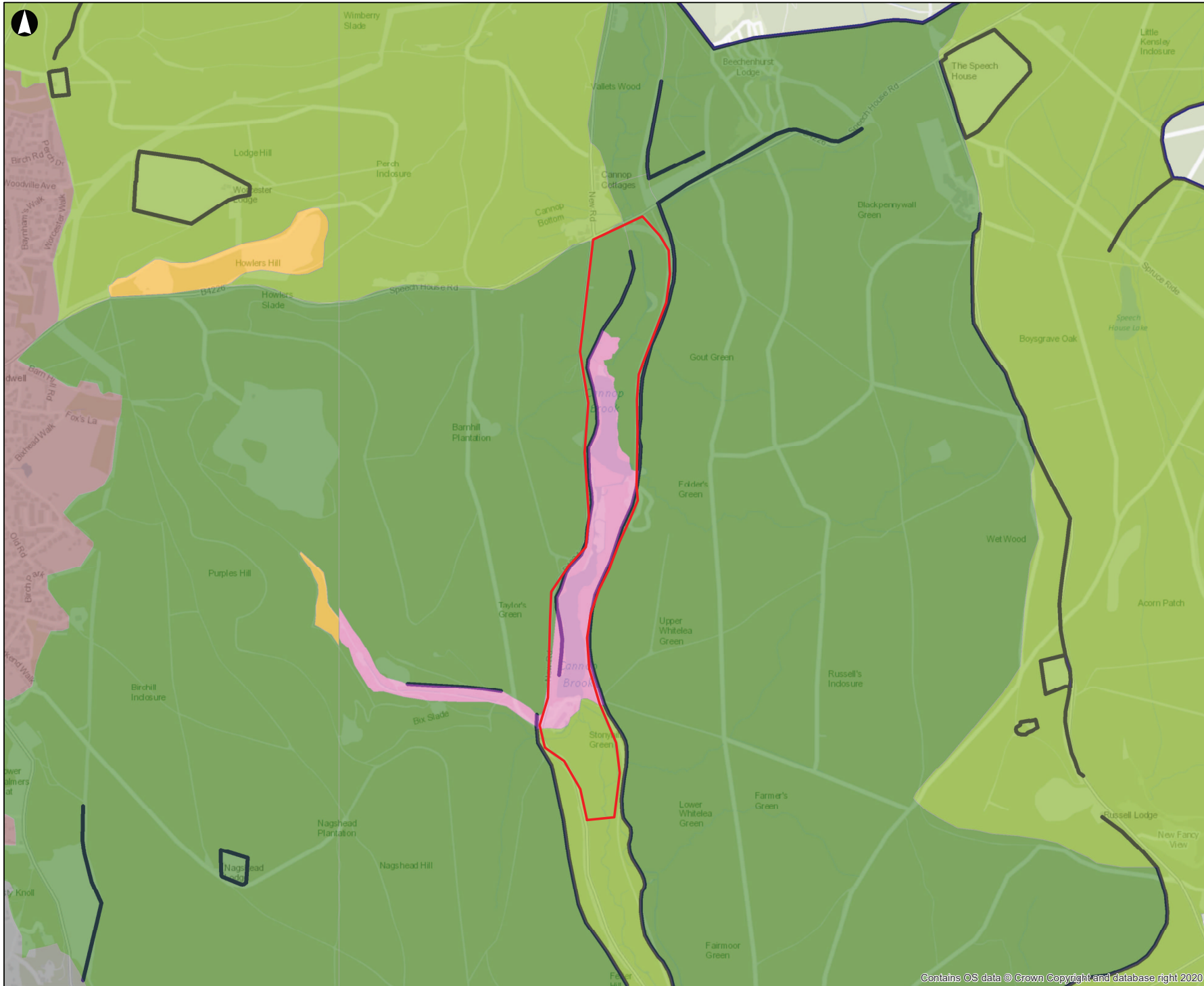
Figure 3: Historic Landscape Characterisation
