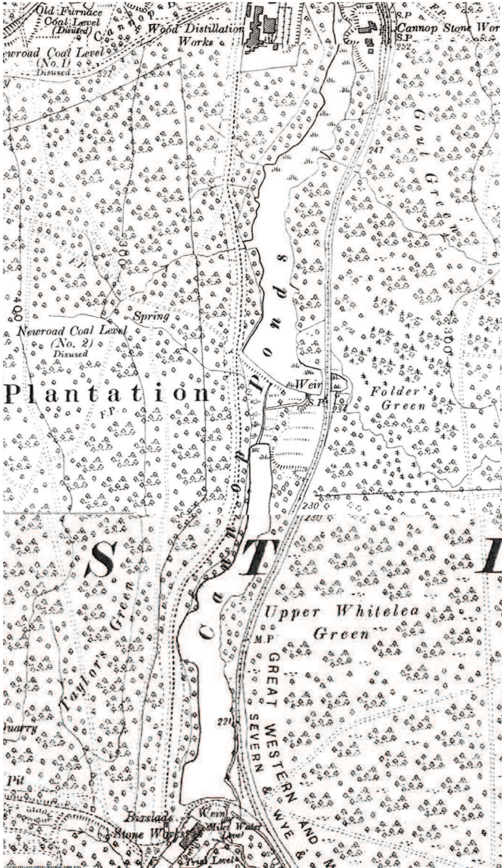
Figure 6: Ordnance Survey 6":mile map of 1924 (used under license from Promap until July 2023)
